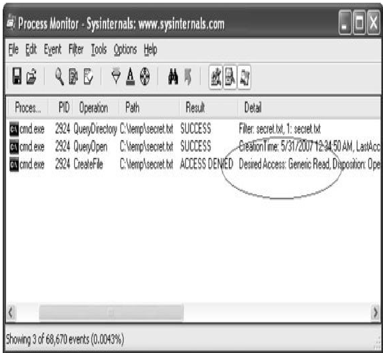
Figure 14-20 Process Monitor log of type c:\temp\secret.txt
