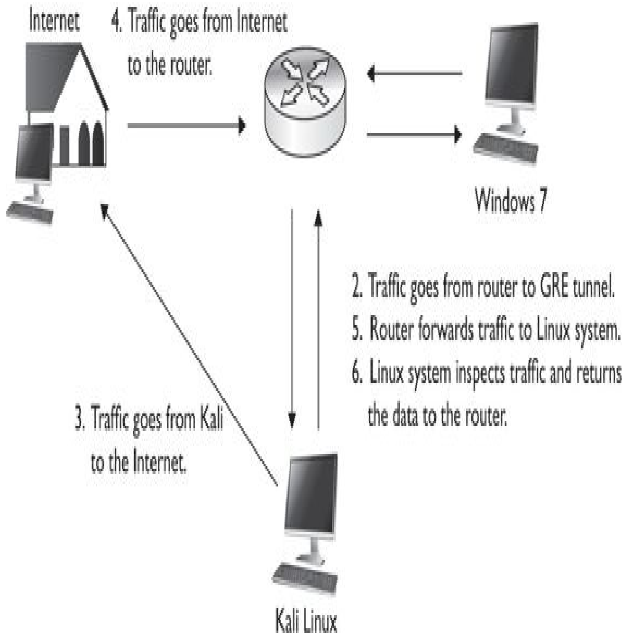
Figure 9-3 The final GRE tunnel workflow
