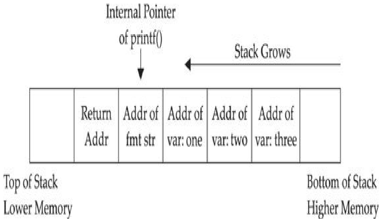
Figure 11-1 Depiction of the stack when printf() is executed
