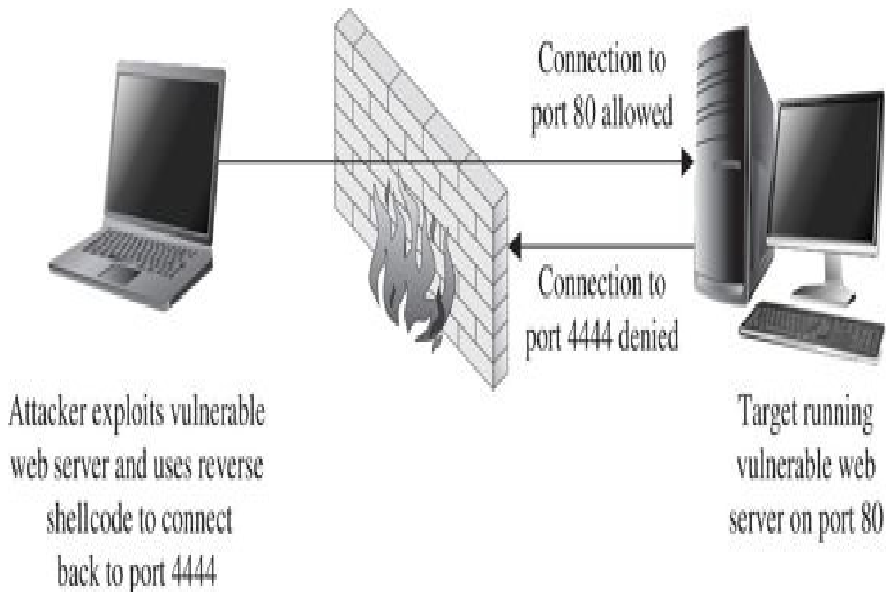
Figure 6-4 Firewall configuration that prevents reverse connecting shellcode
