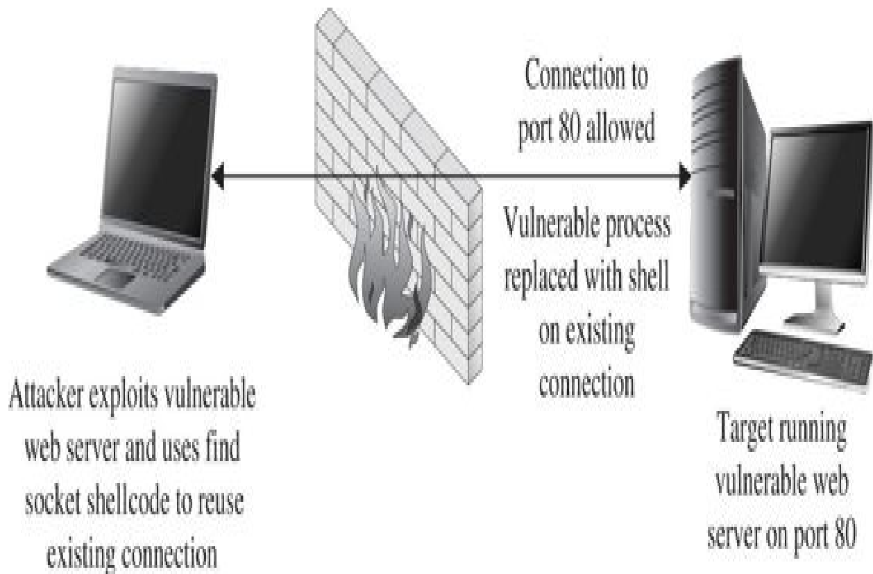
Figure 6-5 Network conditions suited for find socket shellcode
