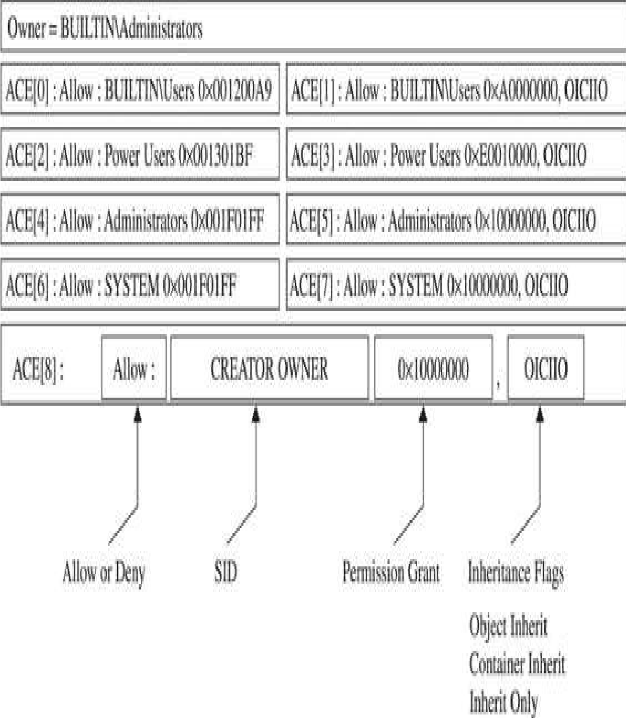
Figure 14-4 C:\Program Files security descriptor
