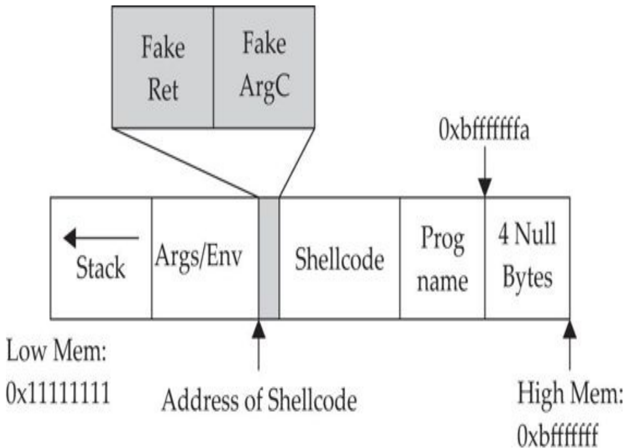
Figure 11-3 Using a fake frame to attack small buffers
