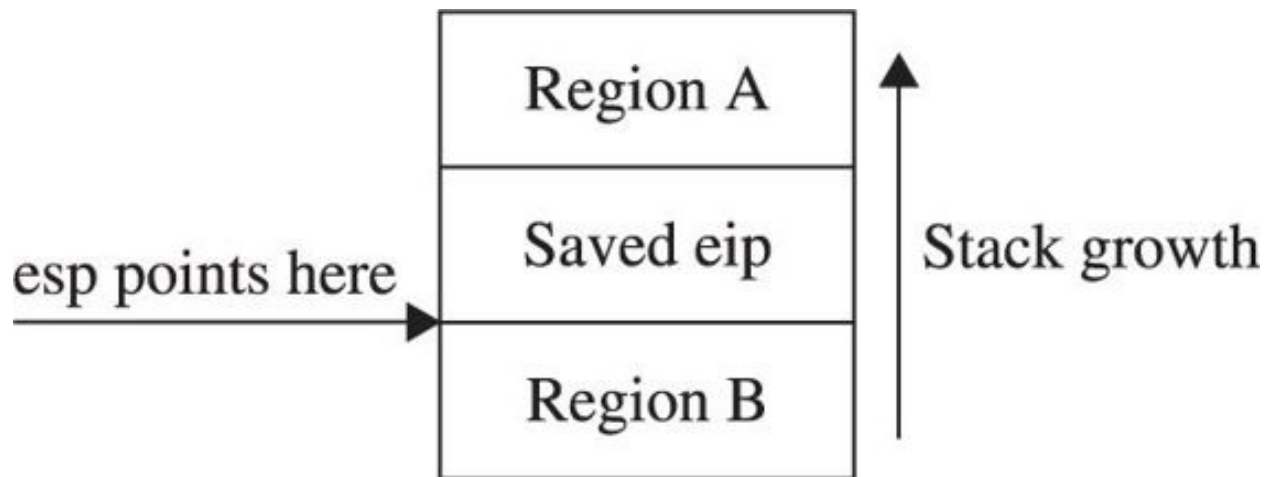
Figure 6-8 Shellcode layout in a stack overflow
