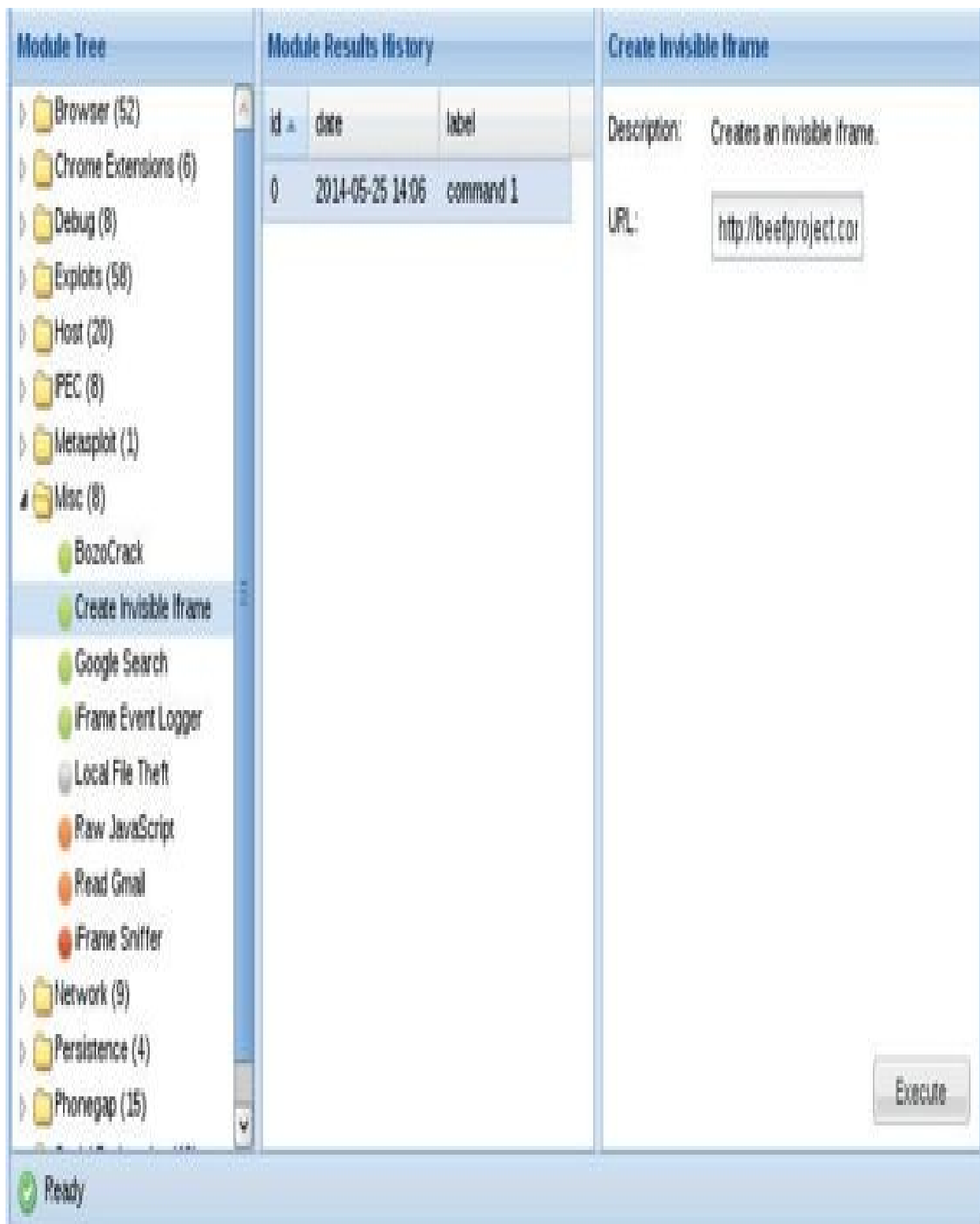
Figure 18-4 The Commands tab display
