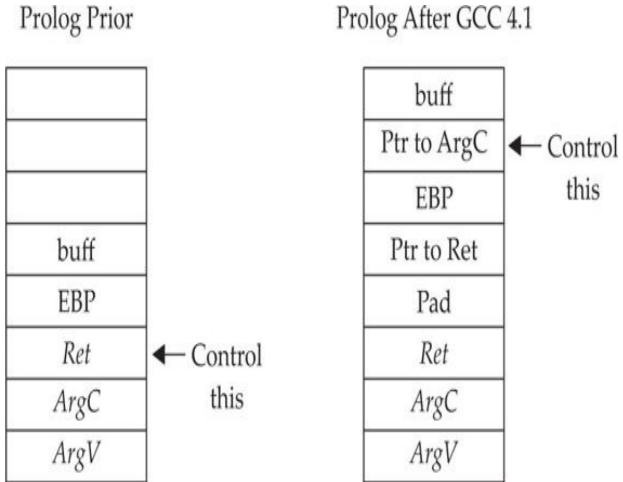
Figure 11-2 Old and new prolog
