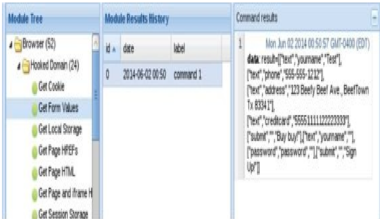
Figure 18-11 Form variables being displayed through BeEF
