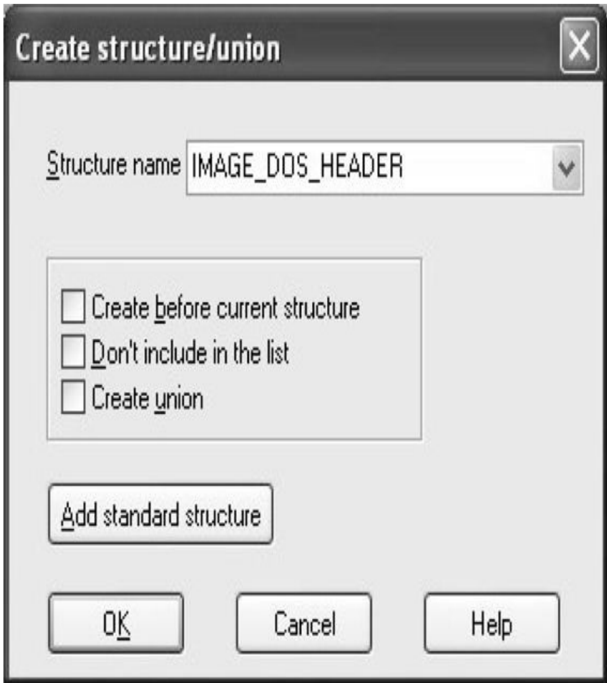
Figure 4-4 Importing the IMAGE_DOS_HEADER structure
