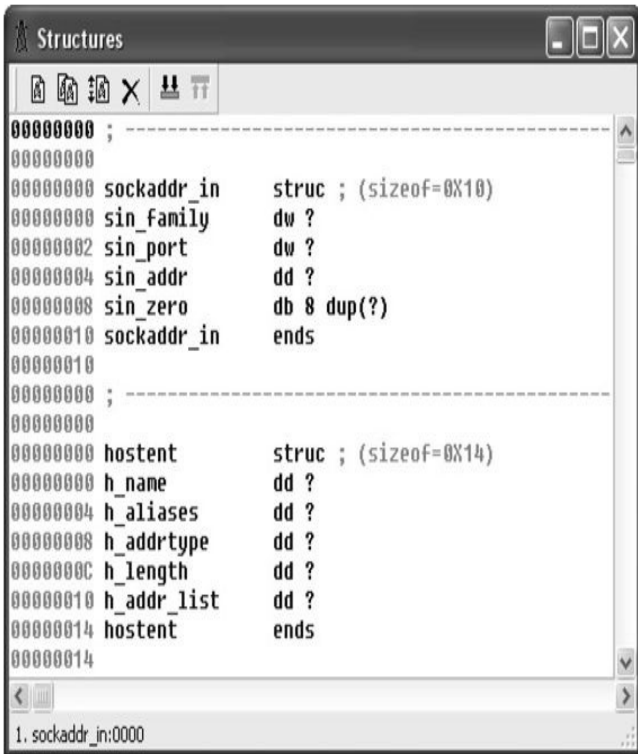
Figure 3-6 IDA Pro Structures definition window
