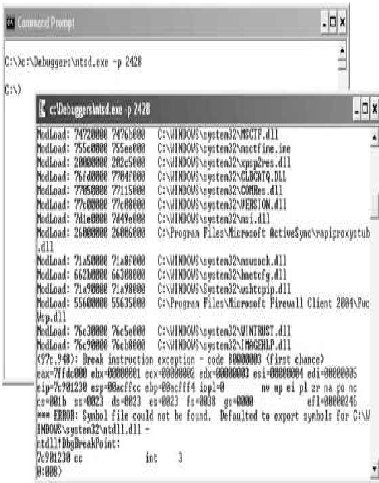
Figure 14-10 Windows debugger
