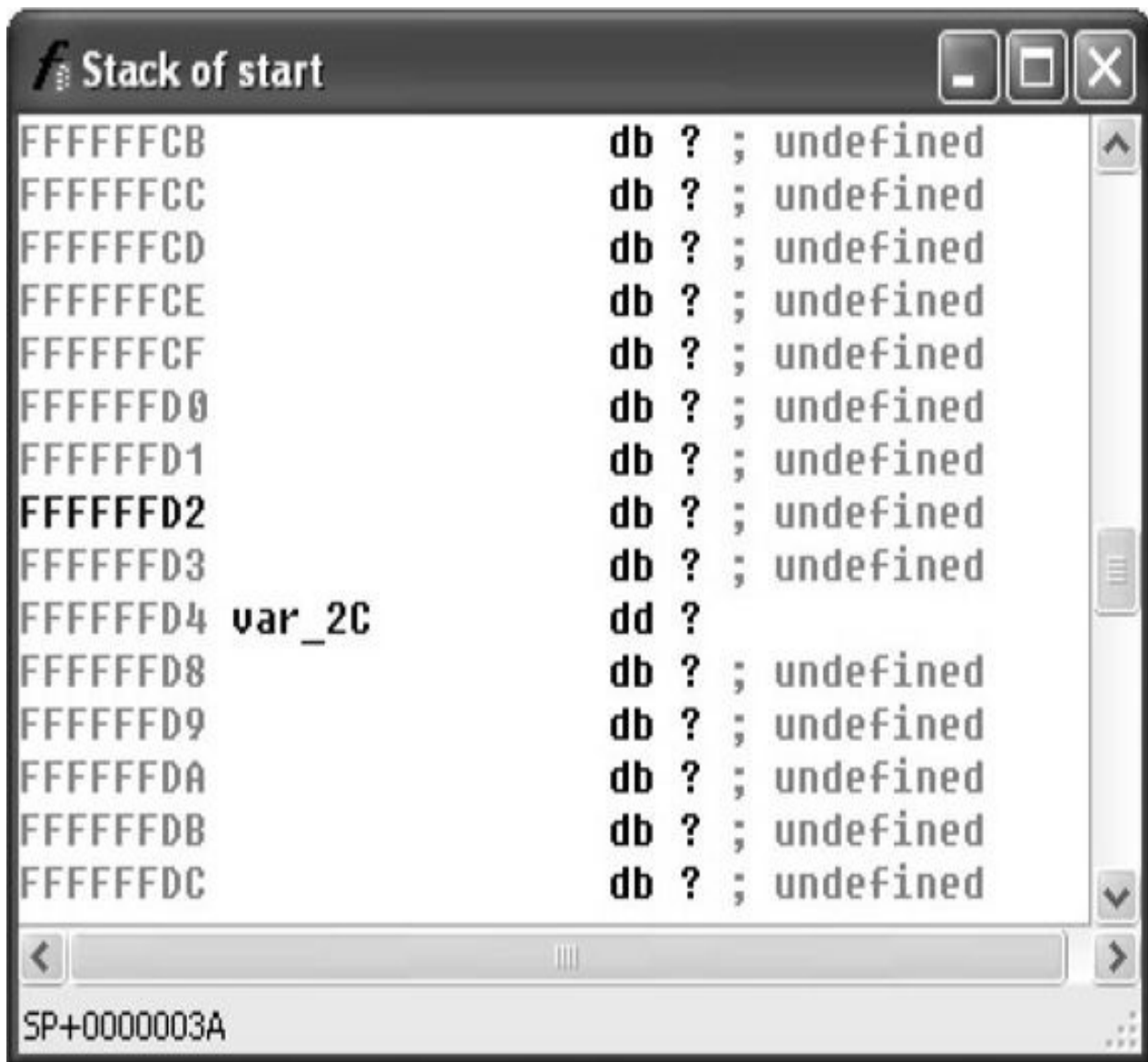
Figure 3-4 IDA Pro stack frame prior to type consolidation
