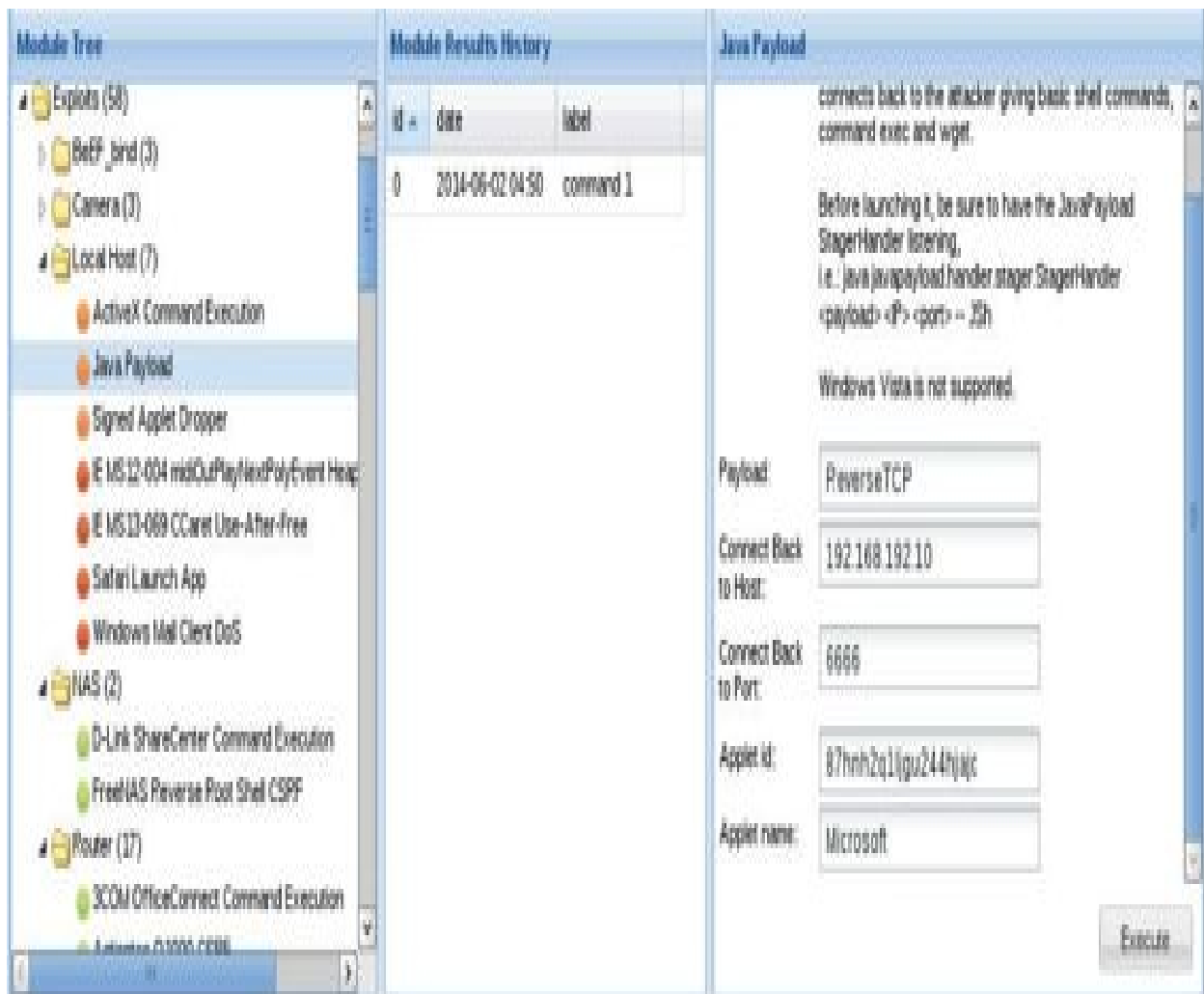
Figure 18-14 The module settings for the Java Payload module
