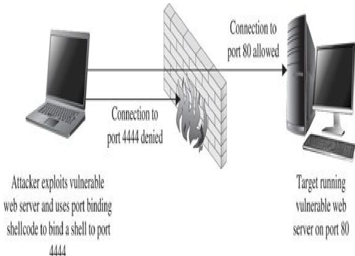
Figure 6-2 Firewall configured to block port binding shellcode
