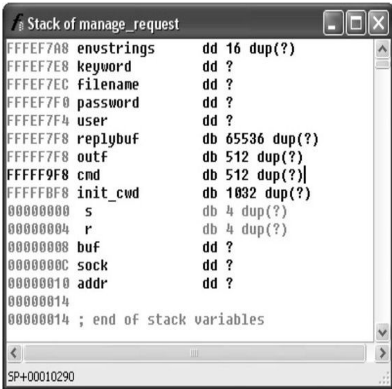
Figure 3-9 The relevant stack arguments for sprintf()
