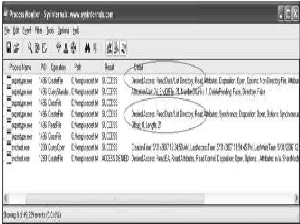
Figure 14-22 Process Monitor log of supertype.exe
