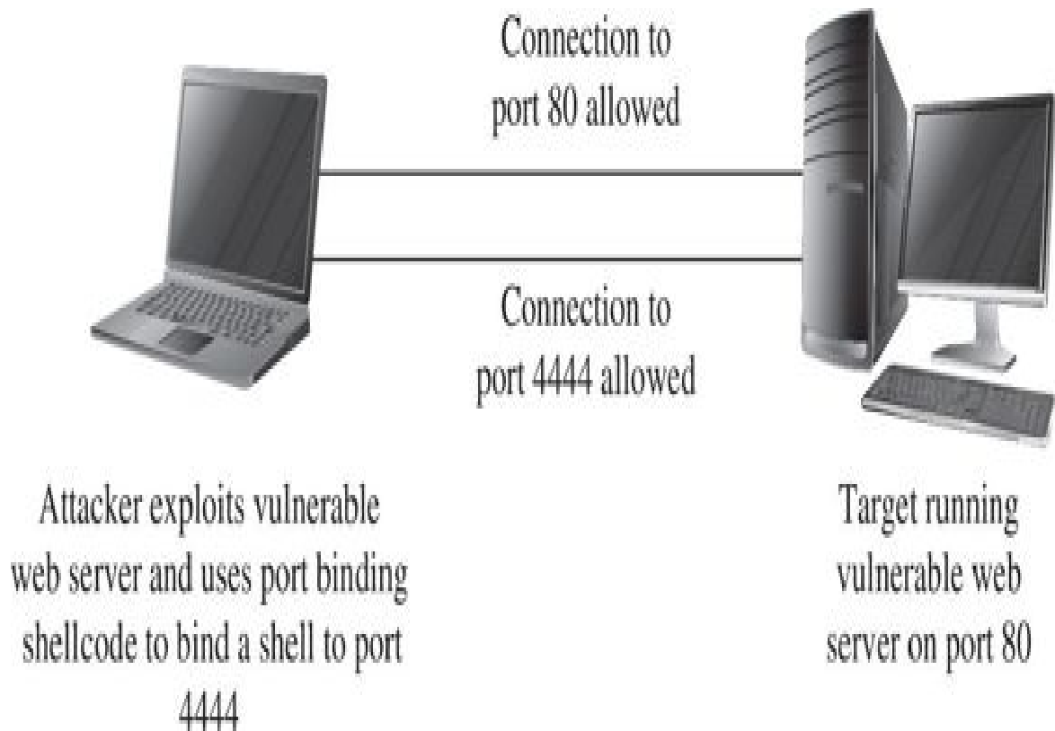
Figure 6-1 Network layout that permits port binding shellcode
