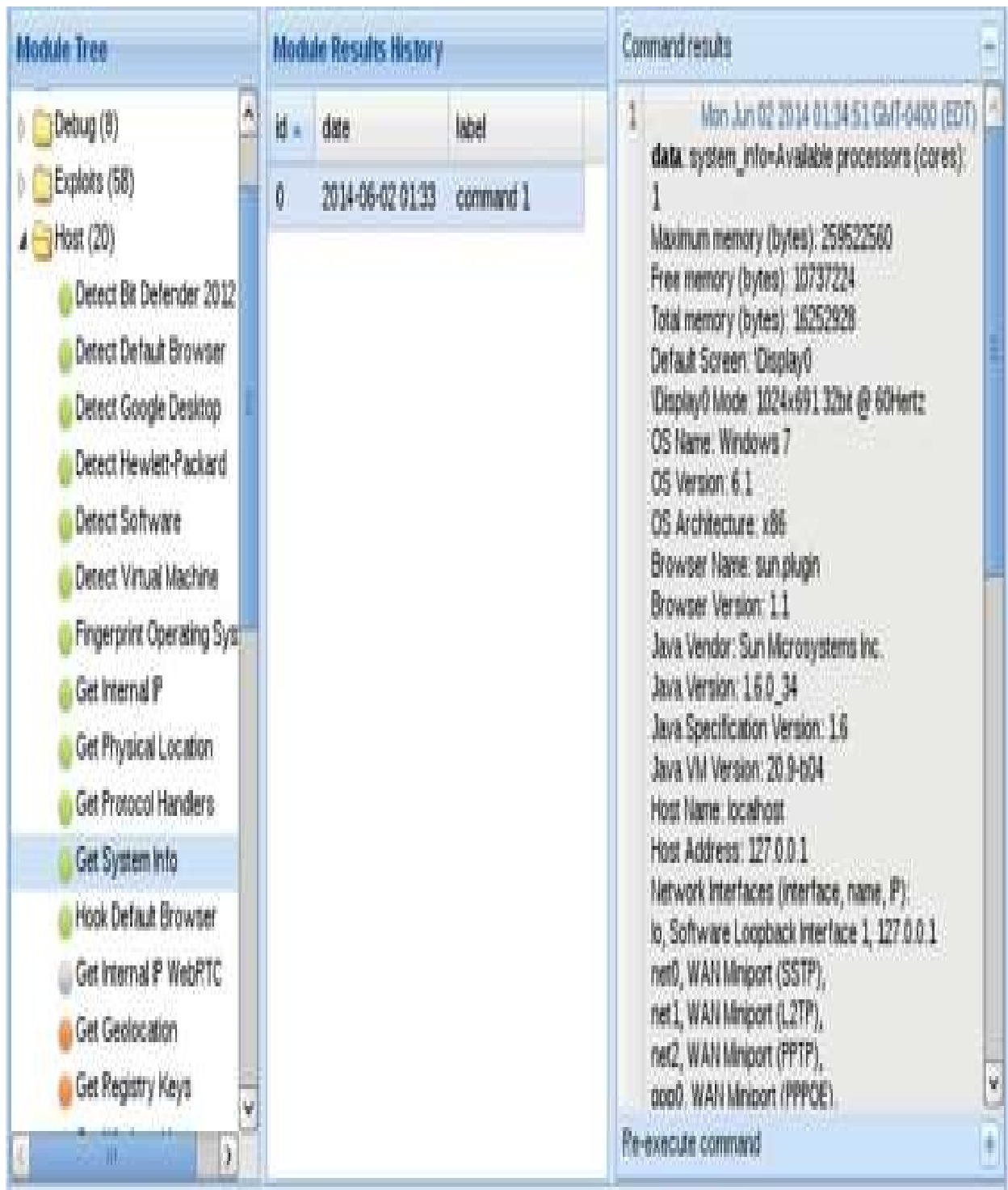
Figure 18-12 The output from the Get System Info module
